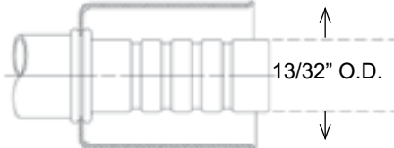
1/2" FITTING FOR NO. 8 HOSE
