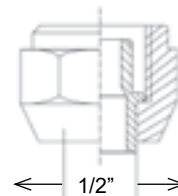
No. 8 3/4"-16 Thread
