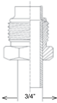
No. 12 1 1/16"-16 Thread
