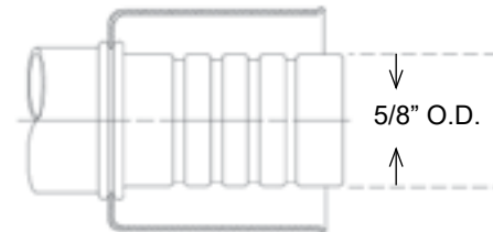
3/4" FITTING FOR NO. 12 HOSE
